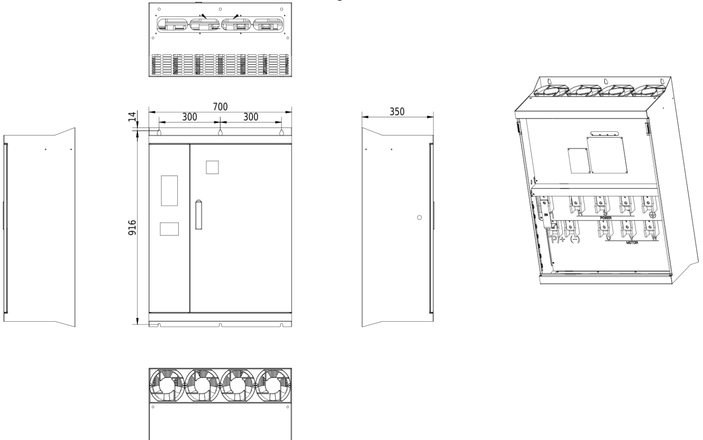
Dimensional drawing V810 - 350kW 4T3500
