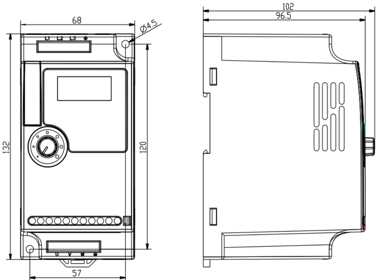
Dimensional drawing A550 Plus - 1,5kW 2S0015
