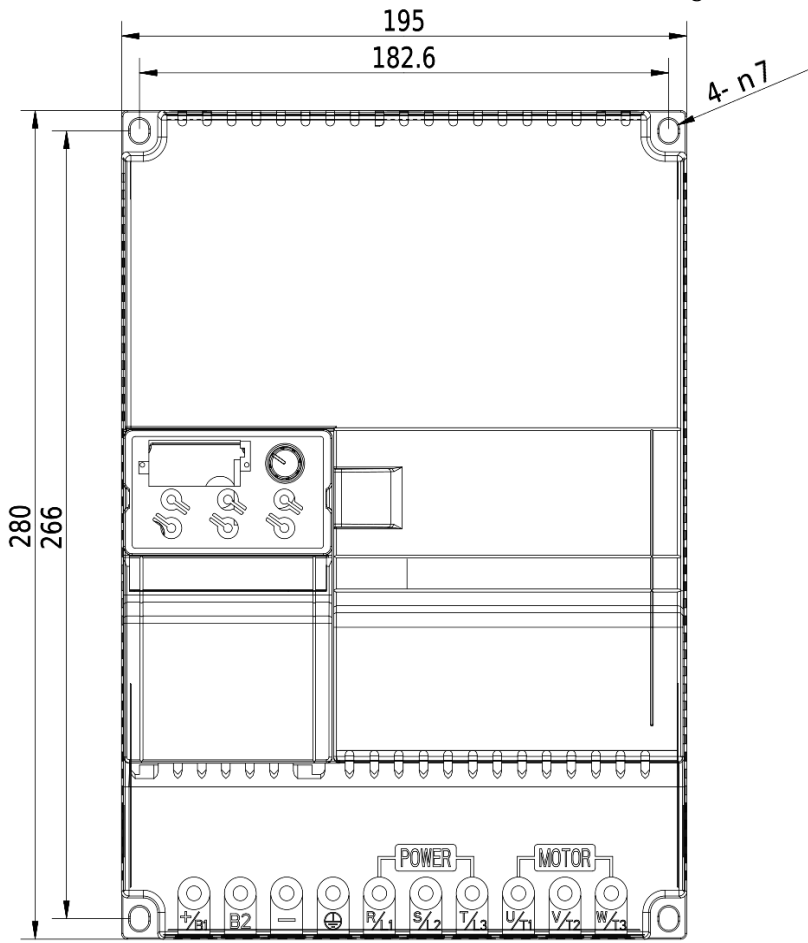
Dimensional drawing V800 - 22kW 4T0220
