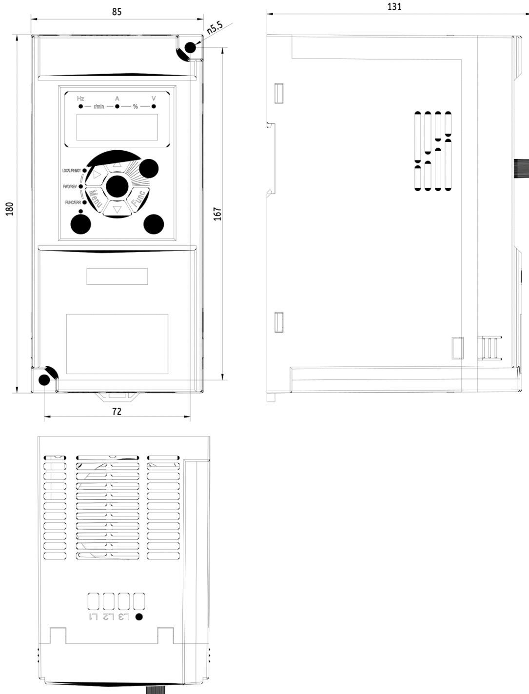
Dimensional drawing V900 - 3kW 4T0030
