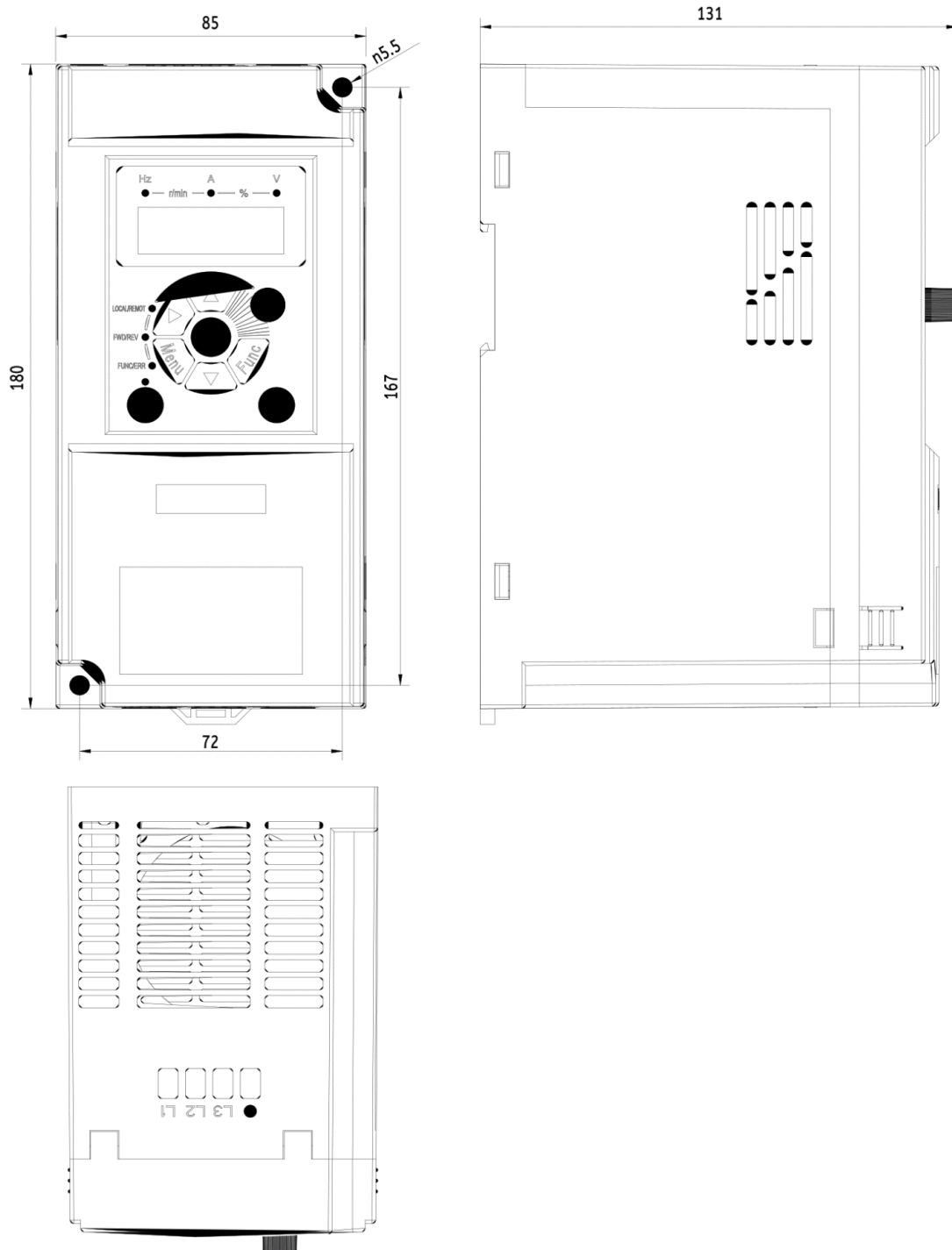
Dimensional drawing V900 - 5,5kW 4T0055
